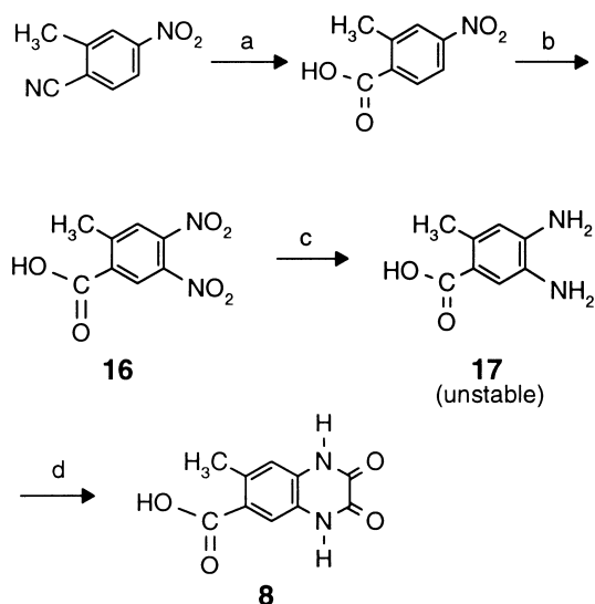
Figure 7. Synthesis of quinoxaline-6-carboxylic acid 8 . Reagents and conditions: (a) \text{H}_2\text{O}_2 , 10% NaOH, reflux; (b) \text{HNO}_3 , \text{H}_2\text{SO}_4 (1:1); (c) \text{NH}_2\text{NH}_2 , \text{Ra}(\text{Ni}) ; (d) \text{EtOCOCO}_2\text{Et} , THF, \text{CH}_3\text{CO}_2\text{H} (cat.), Ar(g), reflux.
