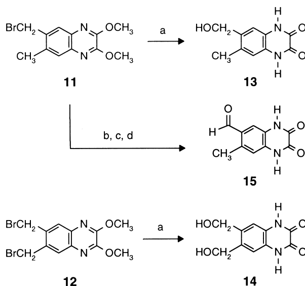
Figure 6. Synthesis of target compounds 13–15 . Reagents and conditions: (a) 1.2 N HCl, \Delta ; (b) \text{C}_6\text{H}_{12}\text{N}_4 ; (c) \text{CH}_3\text{CO}_2\text{H} , reflux; (d) HCl, reflux.
