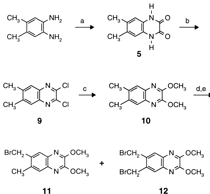
Figure 5. Synthesis of intermediates 11 and 12 . Reagents and conditions: (a) EtOCOCO 2 Et, THF, CH 3 CO 2 H (cat.), Ar(g), reflux; (b) POCl 3 , N,N -dimethylaniline, reflux; (c) CH 3 ONa, CH 3 OH, reflux; (d) NBS, BzOOBz (cat.), CCl 4 , reflux; (e) silica chromatography.
